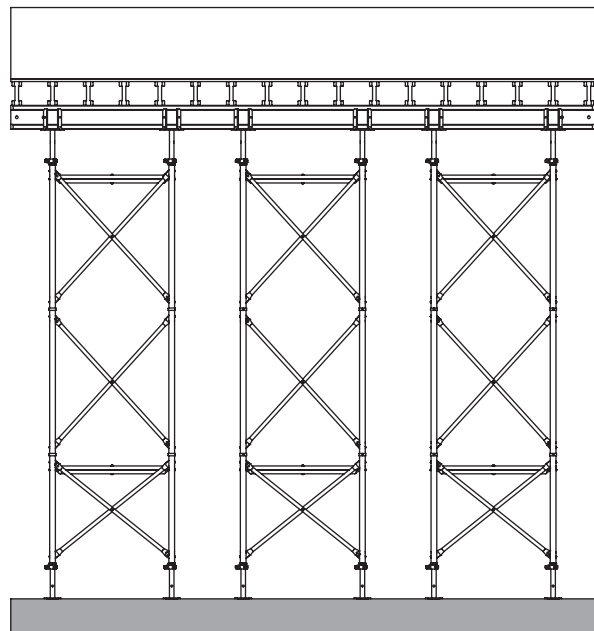
Heavy loads - frames spaced close together
