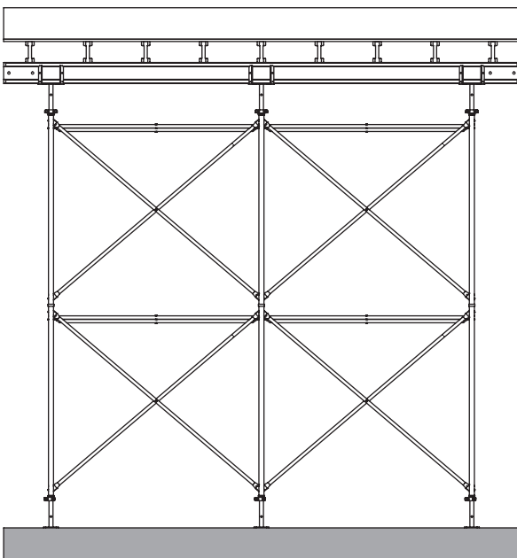
Light loads - frames spaced further apart
