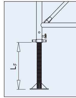
Frames in the top storey 1.8m/1.2m/0.9m 1.8m/1.2m 0.9m
